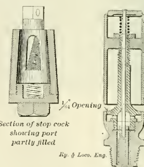
DETAILS OF "BACK-UP" HOSE DEVICE USED ON THE MICHIGAN CENTRAL RY.
